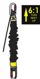
Cam Disengaged For lowering
